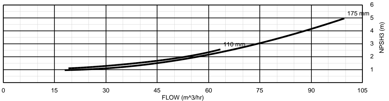
Testbay curve - water duty
